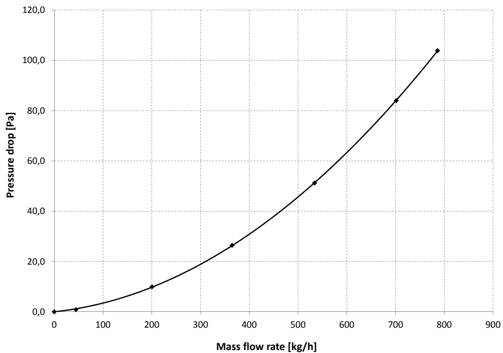
Figure 5: Druckverlust des Kollektors SV Professional measured pressure drop of the collector SV Professional
