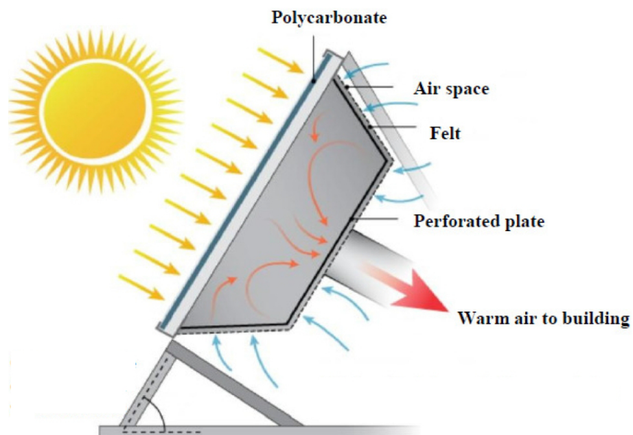
Figure 2: Abbildung des Kollektors (Quelle: Herstellerdokumentation) - Picture of the collector (Source: Manufacturers documentation)
