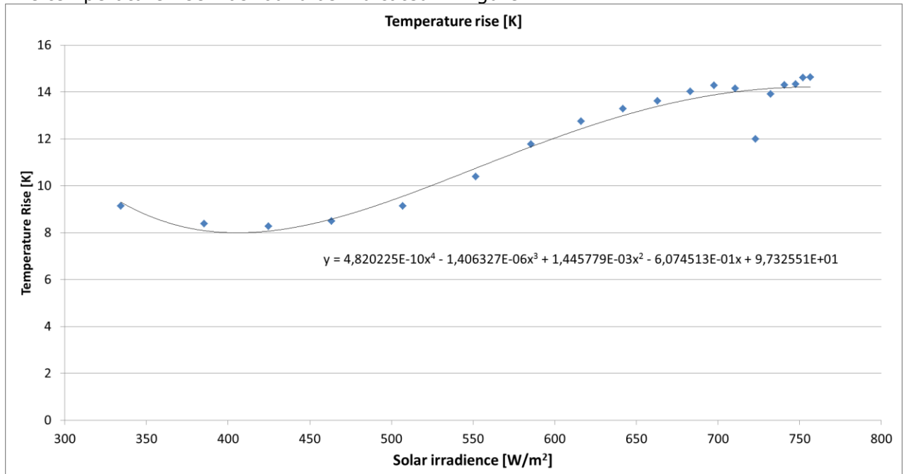
Figure 2 - Temperature rise
