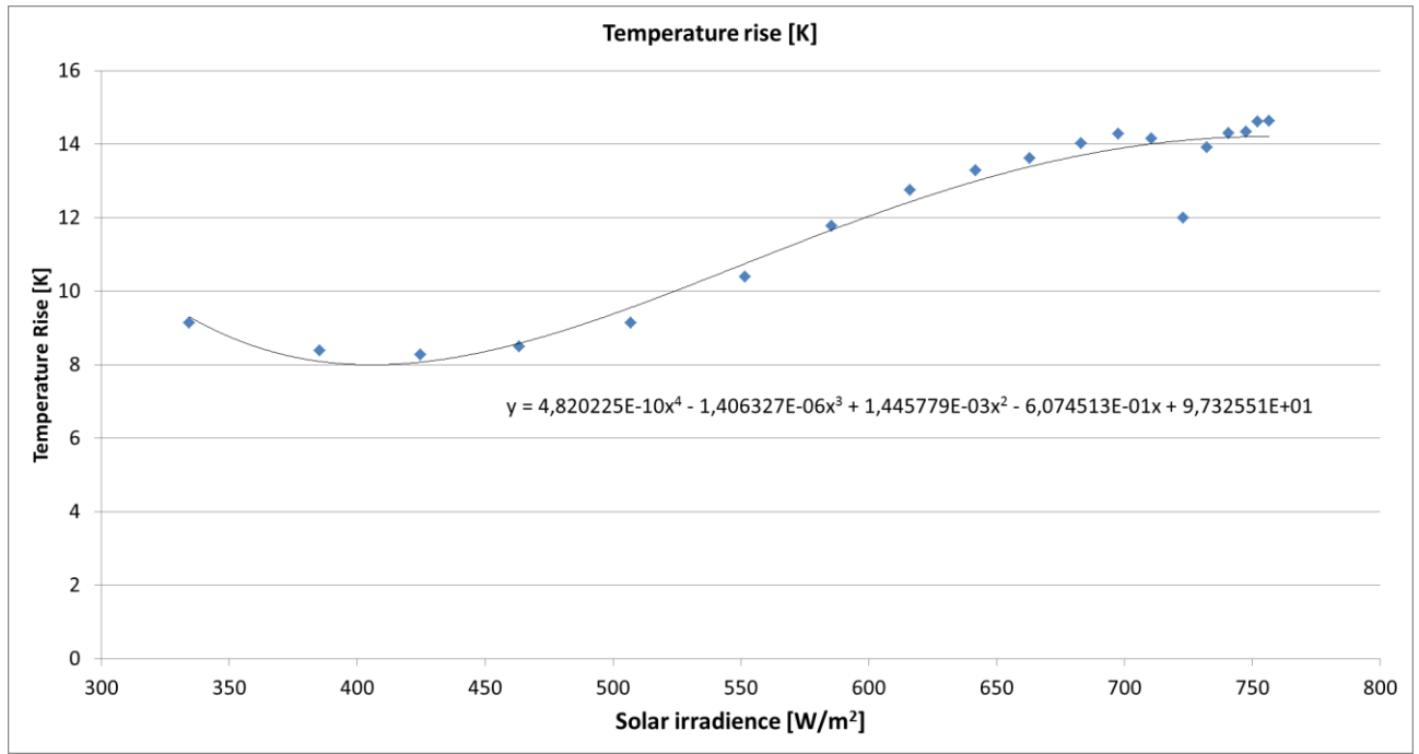
Figure 4 - Temperature rise
