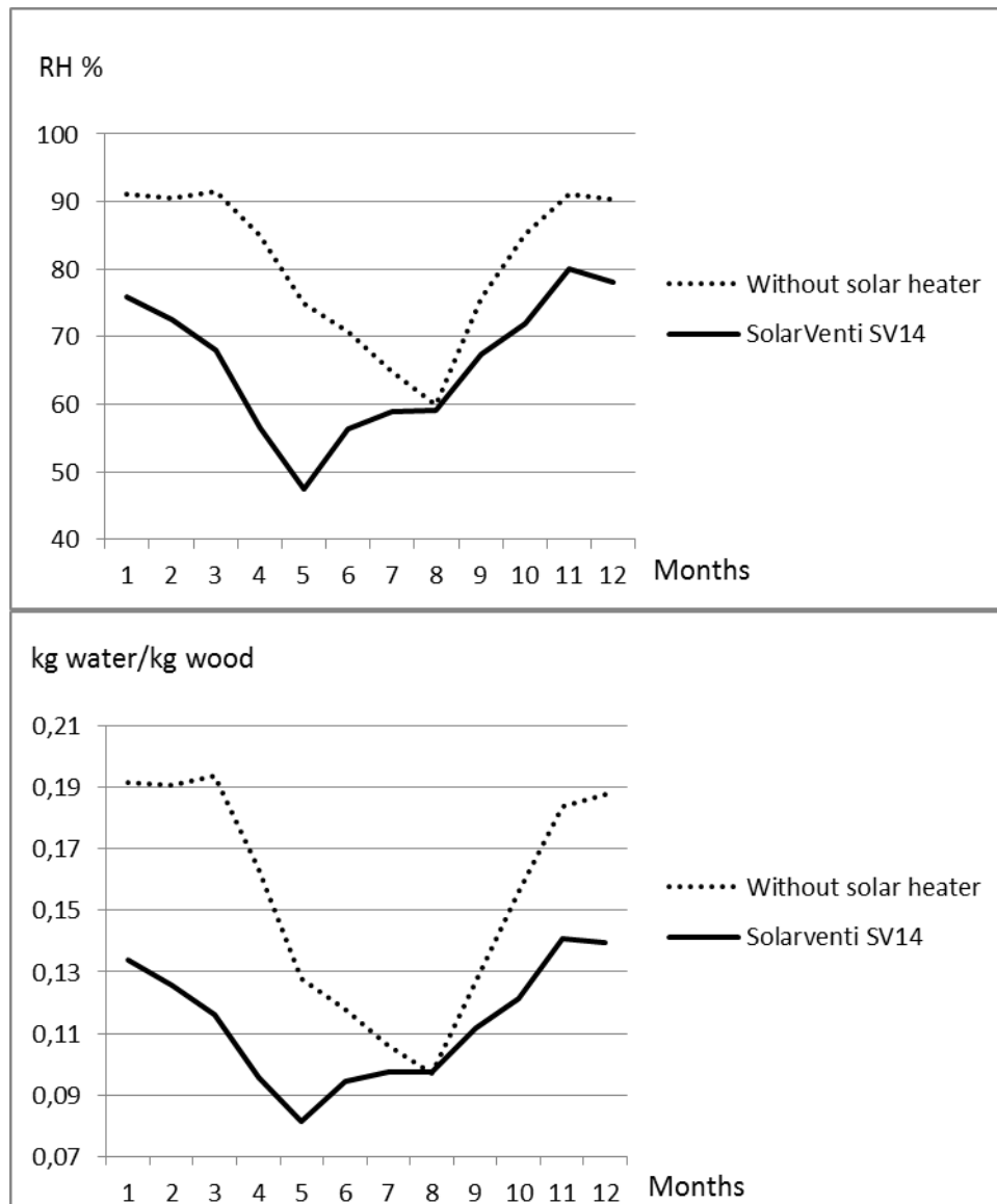
Figure 5 - Simulation results
